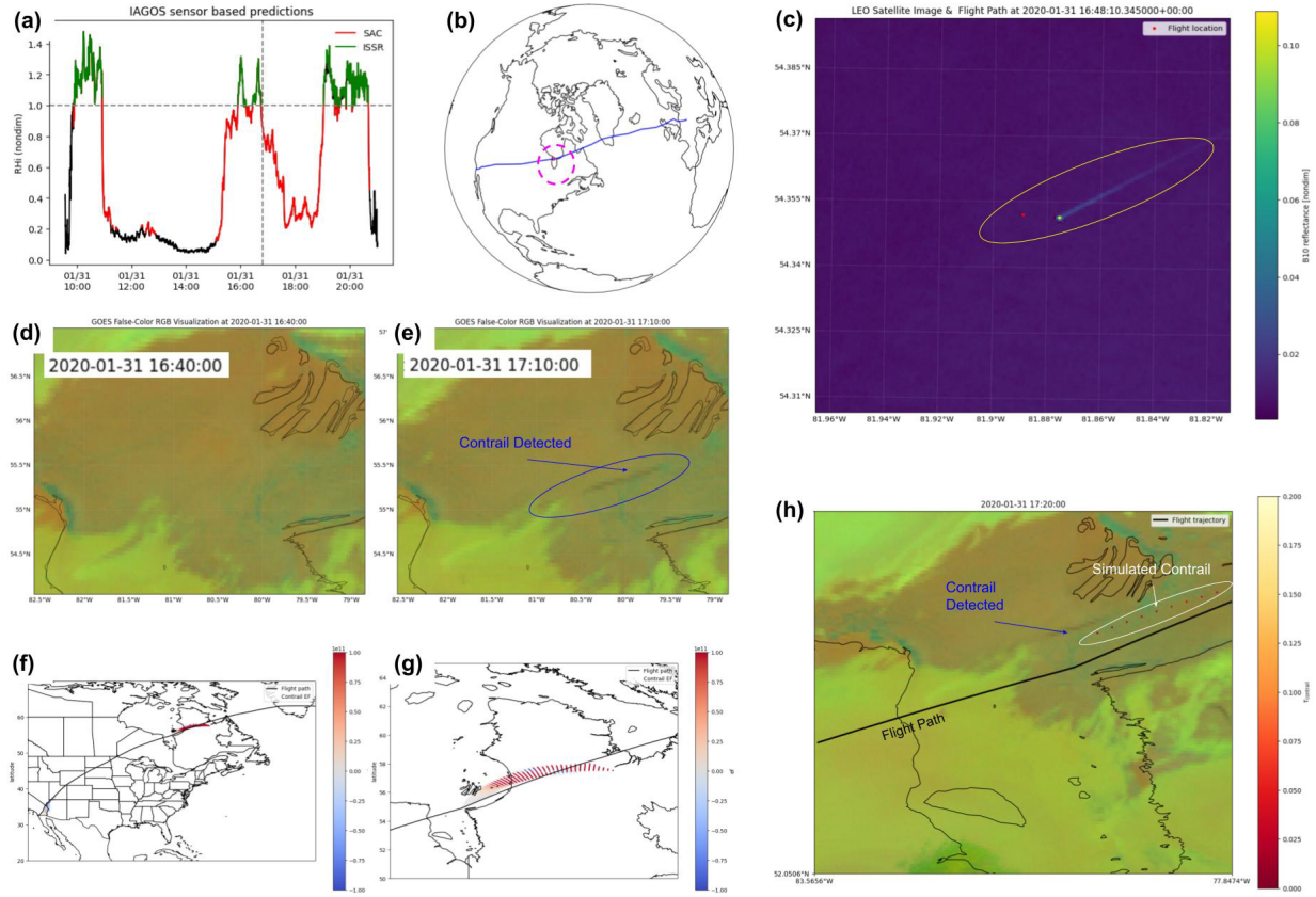
Figure 3. Methods visual flow. End-to-end workflow from along-track humidity to satellite intersection, detection, and CoCiP validation. (a) In-track IAGOS RH i along the flight, indicating segments satisfying SAC and ISSR criteria. (b) Global projection showing the flight path intersecting a LEO swath. (c) LEO image at the intersection, with the young contrail highlighted in yellow. (d-e) Corresponding GEO (GOES-16) image at the intersection time (contrail too small to resolve) and 30 min later when the contrail becomes visible at GEO resolution. (f-g) CoCiP-simulated contrail overlaid on a map; red denotes warming EF. (h) CoCiP simulation overlaid on the GEO image and flight track, used to compare observed contrails (blue tones) with simulated contrails (white highlight).
