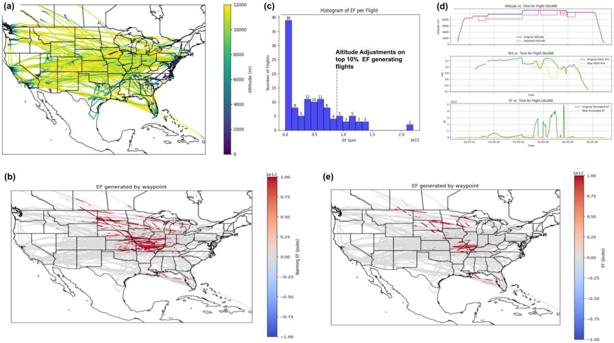
Figure 4. Navigational contrail mitigation case study. Results from a 200-flight contrail-mitigation rerouting case over a 12-h nighttime period in the USA. (a) Trajectories and altitudes of the 200 flights. (b) CoCiP-simulated heat map of contrail energy forcing (EF) per flight using ERA5 RHi with exponential boosting; red denotes warming. (c) Histogram of EF across flights; altitude adjustments are applied to the top 10% of flights by EF. (d) Example flight showing applied altitude changes, the resulting RHi at the new altitude, and the reduction in EF. (e) Post-mitigation CoCiP heat map demonstrating reduced warming EF for the top 10% EF flights.
