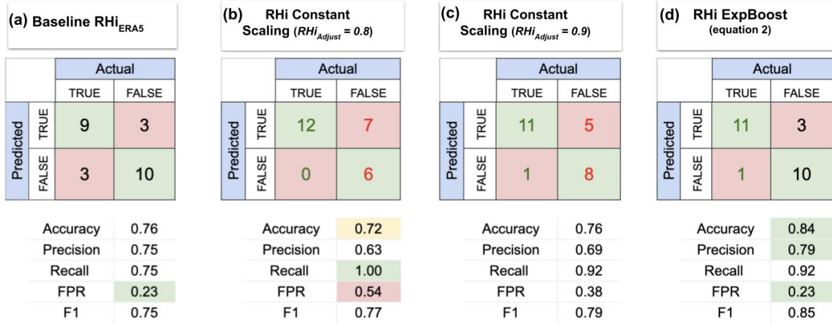
Figure 6. Confusion matrices and metrics under RHi scaling. Panels show confusion matrices and summary metrics for (a) baseline, (b) constant scaling = 0.8, (c) constant scaling = 0.9, and (d) exponential boost. Accuracy and F1 were closely matched across panels (e.g., baseline \approx 76\%/75\% ; exponential boost \approx 84\%/85\% ), indicating a balanced evaluation set. Constant scaling increased recall (fewer false negatives) but at the cost of higher false positives, with the trade-off growing as the scale factor increased. In contrast, the exponential boost improved both accuracy ( 76\% \Rightarrow 84\% ) and F1 ( 75\% \Rightarrow 85\% ) simultaneously, reflecting better balanced detection. Notably, the false-positive rate ( \approx 23\% ) remained largely unchanged across scalings, indicating that RHi scaling alone could not reduce false positives and that other factors (e.g., unresolved vertical structure, shear, timing/geo-registration) likely dominated.
