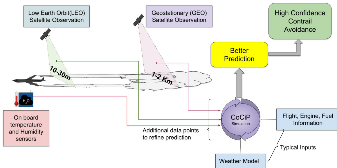
Figure 1. Hypothesis Diagram. Data fusion (IAGOS, LEO, GEO) validates CoCiP lifecycle predictions. Along-track IAGOS in situ RH i measurements are integrated with low-Earth-orbit (LEO) and geostationary (GEO) satellite observations to calibrate CoCiP inputs and validate per-flight contrail life cycles, enabling higher-confidence contrail-avoidance strategies.
