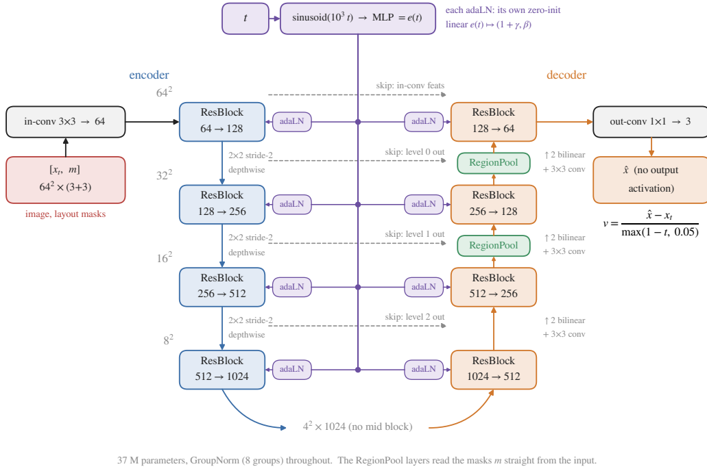
Figure 1: The velocity network. Input: x_t with the three layout-mask channels. Four encoder levels (ResBlock doubling the channels, then a 2 \times 2 stride-2 depthwise convolution), a bare 4^2 \times 1024 tensor with no mid block, four decoder levels (bilinear \uparrow 2 and a 3 \times 3 convolution, concatenation of the skip, ResBlock halving the channels). Skips run from the input of each encoder level to the decoder level after its upsample (Fig. 3). Region pooling follows the decoder levels producing 16^2 and 32^2 . Time enters every ResBlock through adaLN-Zero; the output is \hat{x} with no activation, and the velocity is derived from it.
