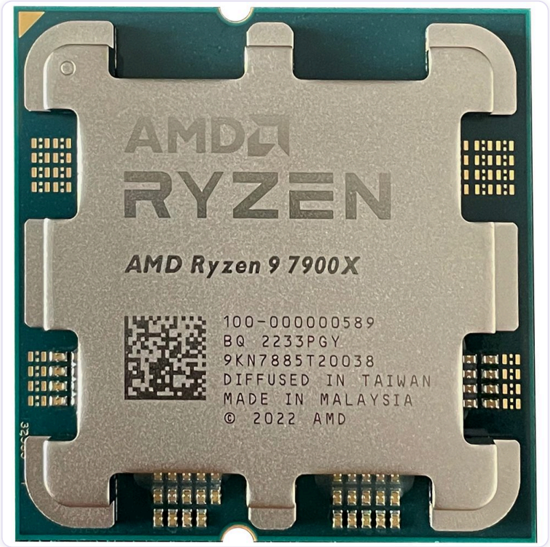
A desktop Ryzen 9 processor. The metal lid (IHS) spreads heat; underneath it sit the chiplets shown in the next photo. Photo: CristoCalis, CC BY-SA 4.0 via Wikimedia Commons.
