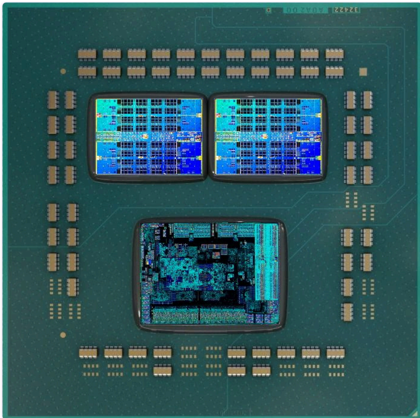
Inside a Ryzen: two CPU core chiplets (top) and one I/O die (bottom) on a single package. Building it this way is why AMD can offer more cores for less money than a single giant die would allow — and it is the same idea, scaled up, inside EPYC and Instinct. Photo: Zenmaster2021, CC BY-SA 4.0 via Wikimedia Commons.
