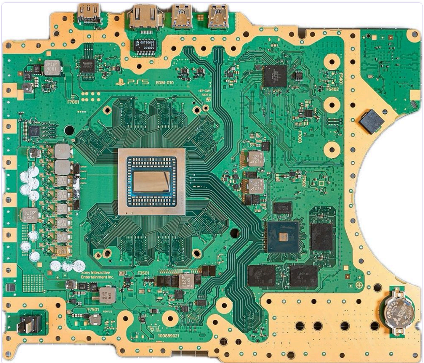
A PlayStation 5 motherboard. The large square package in the centre is a custom AMD APU — Zen 2 CPU cores and an RDNA 2 GPU on one die, designed by AMD specifically for Sony. The dark chips around it are GDDR6 memory. Photo: Fritzchens Fritz, CC0 via Wikimedia Commons.
