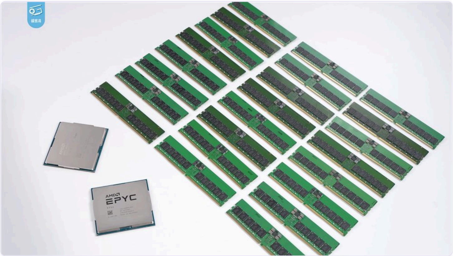
An AMD EPYC server processor beside the memory it feeds — 24 DDR5 modules for a dual-socket server. The chip is roughly the size of a matchbox lid; the memory around it is what an AI or database workload actually eats. Photo: 极客湾Geekerwan, CC BY 3.0 via Wikimedia Commons.
