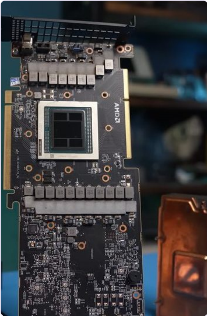
What a data-centre AI GPU physically looks like — an older AMD Instinct card with its cooler removed. Note the large central die surrounded by memory stacks, and no display outputs at all : this is a pure compute engine. The MI455X follows the same idea at roughly 20× the scale. Photo: Мой Компьютер, CC BY 3.0 via Wikimedia Commons (cropped).
