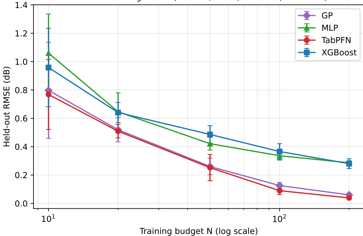
Insertion-loss regression (mean \pm 1 SD; 10 seeds, N=50: 30)
