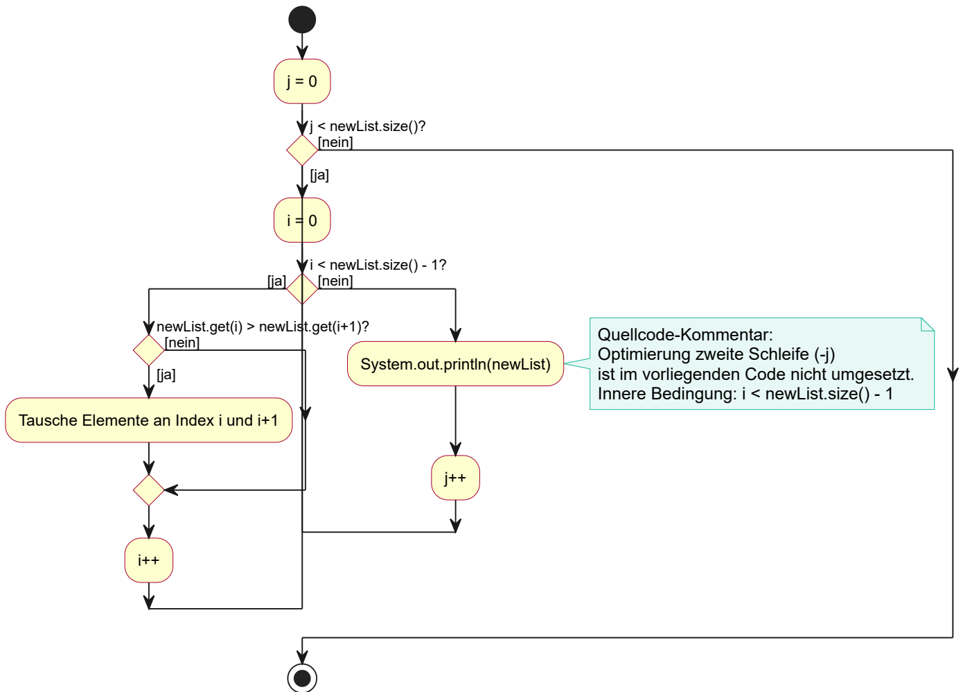
BubbleSort ueber newList
