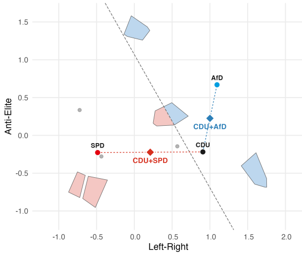
(a) Illustration: Coalition policy positions and random cells of voters’ locations
