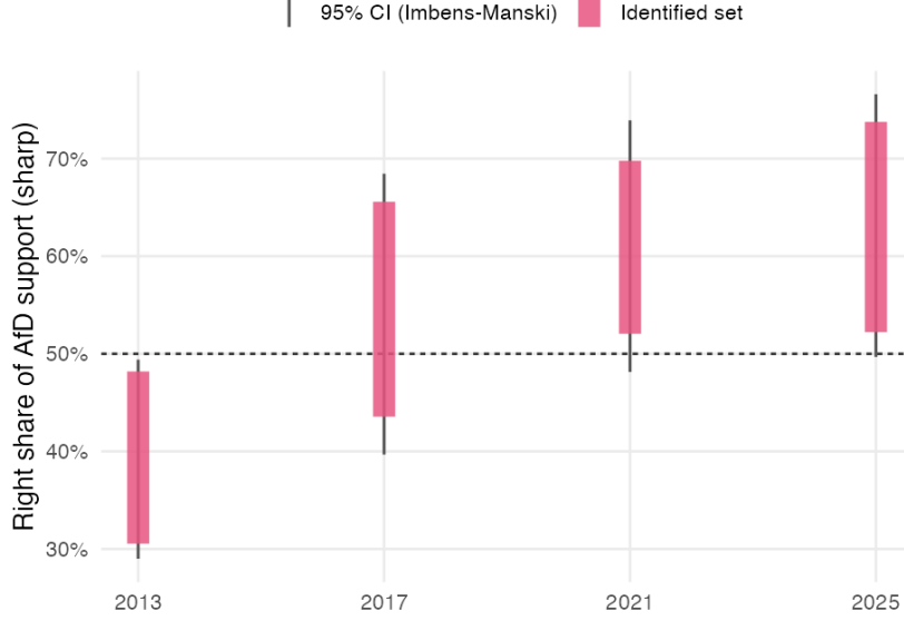
Bars show the sharp identified set for the Right share of AfD support, \theta_{Right} , in the main specification without second-choice moments, aggregated over East and West with AfD-vote weights within each bootstrap replication. Whiskers are 95% confidence intervals for the parameter following (Imbens and Manski, 2004). Endpoint standard errors are obtained from a nonparametric bootstrap ( B = 100 ) that resamples municipalities with replacement within state-election strata and re-solves the full linear programme on each draw.
