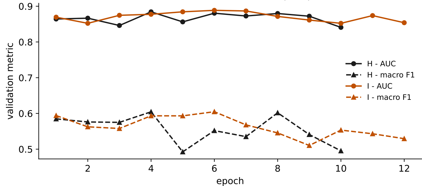
Task 9 - validation discrimination per epoch
