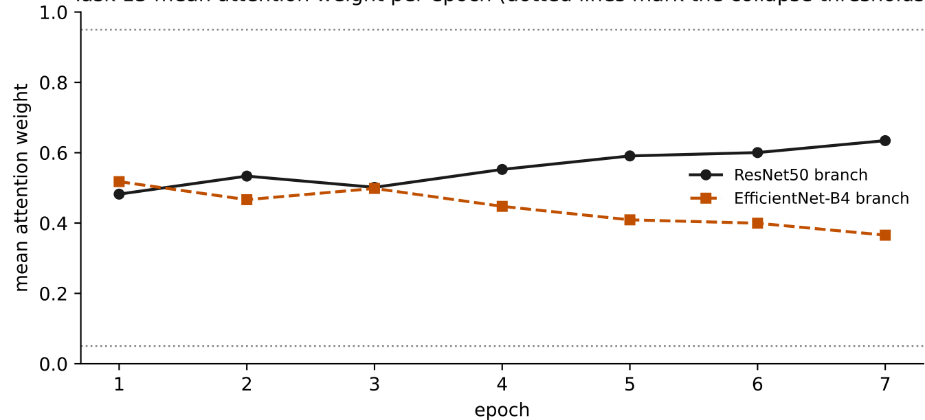
Task 13 mean attention weight per epoch (dotted lines mark the collapse thresholds)
