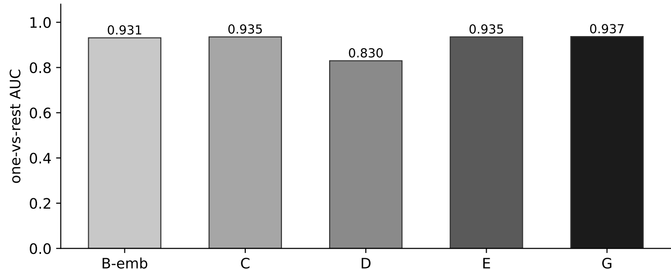
Canonical test set, N = 1331 - Pre-Plus class
