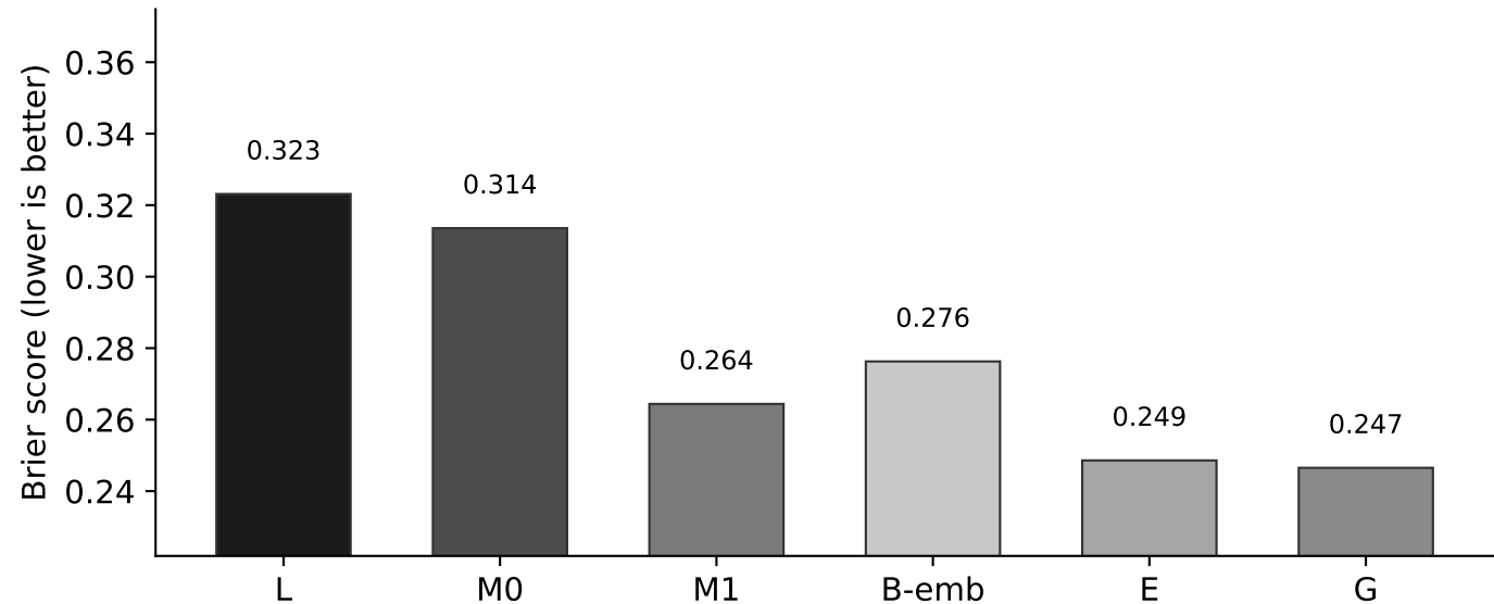
Canonical test set, N = 1331 - Brier score
