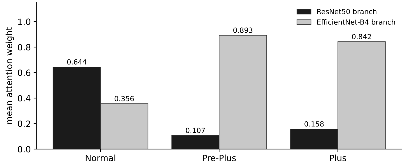
Task 13 - mean attention weight by true class
