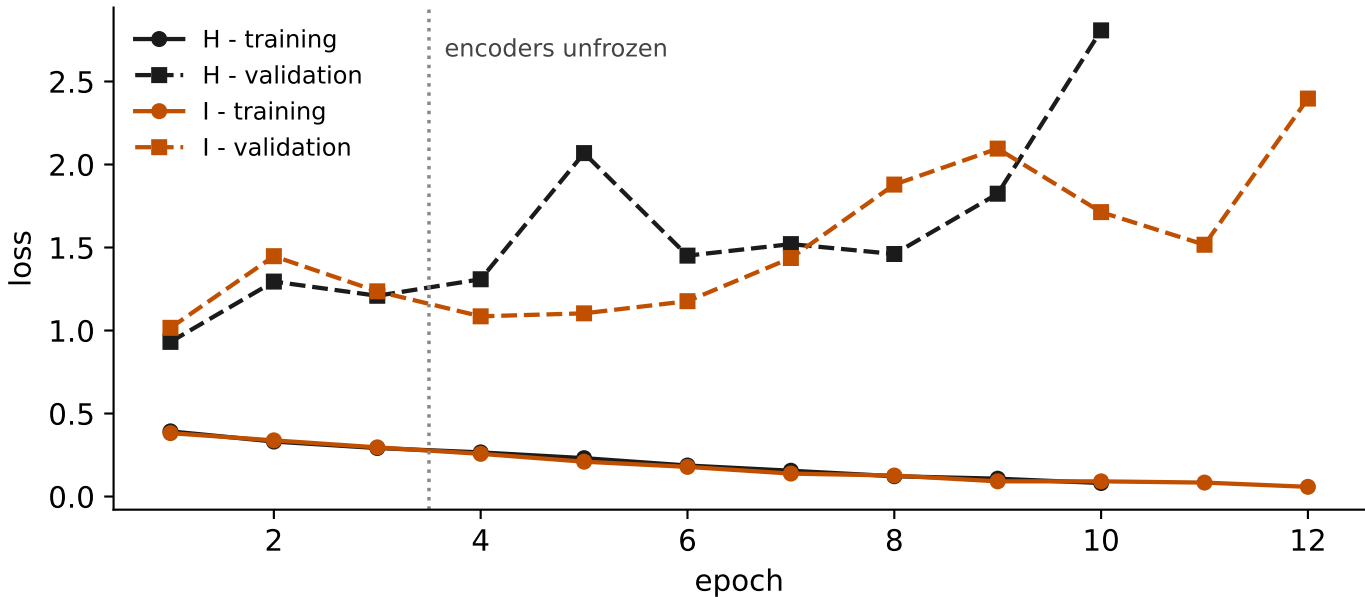
Task 9 - loss per epoch (encoder tails unfrozen after epoch 3)
