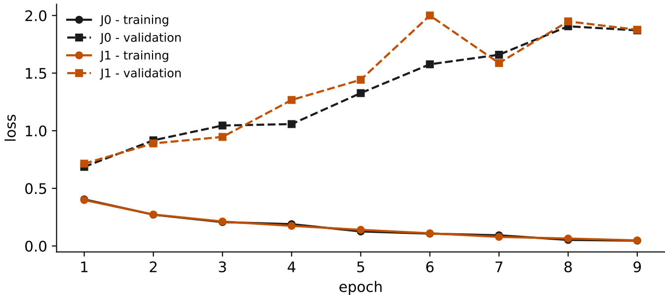
Task 10 - loss per epoch (frozen embeddings, head only)
