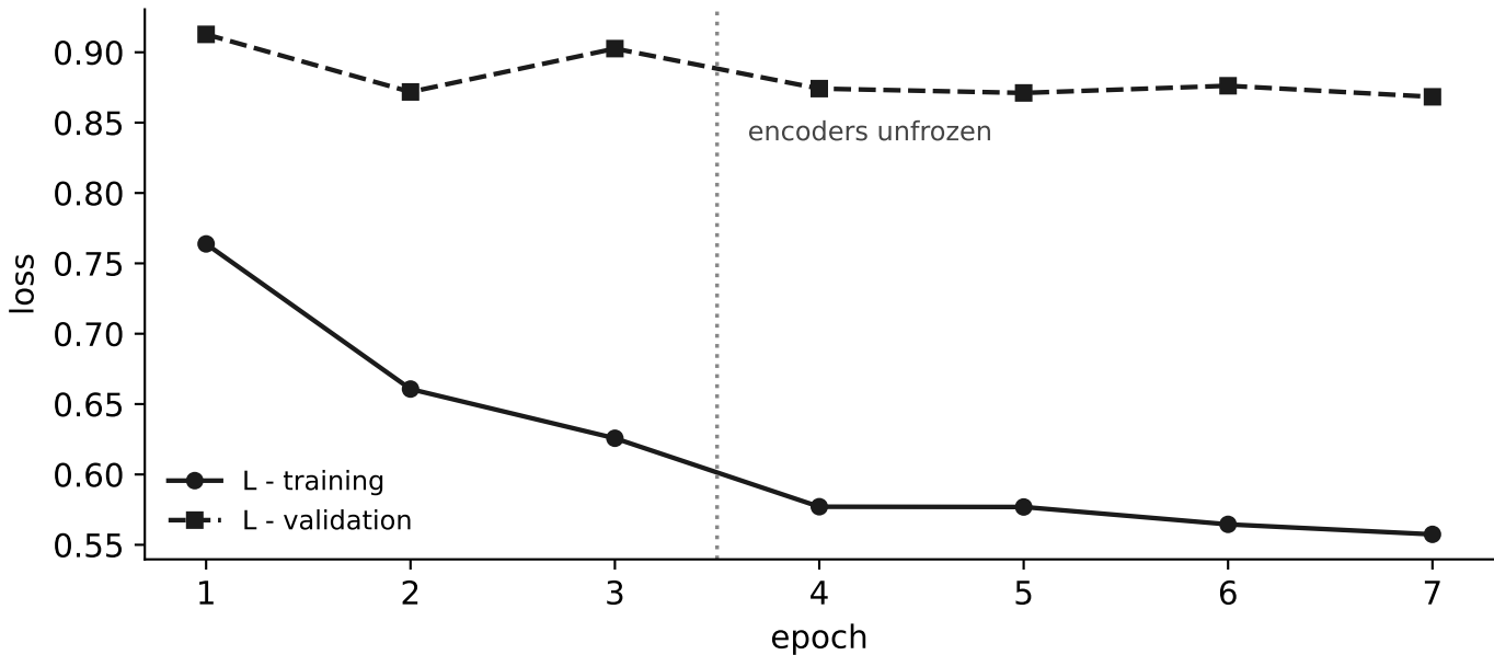
Task 13 - loss per epoch (backbones unfrozen after epoch 3)
