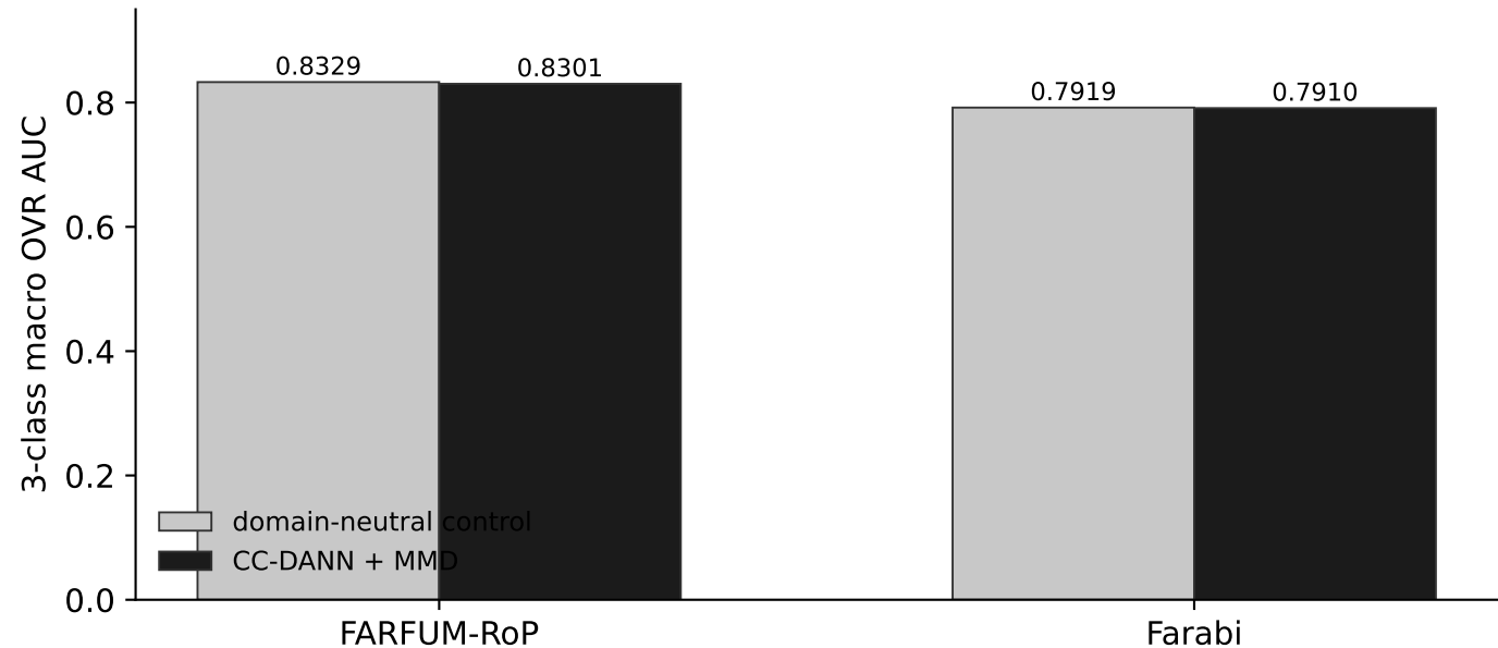
Task 12 - held-out source, three-class AUC
