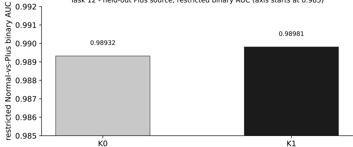
Task 12 - held-out Plus source, restricted binary AUC (axis starts at 0.985)
