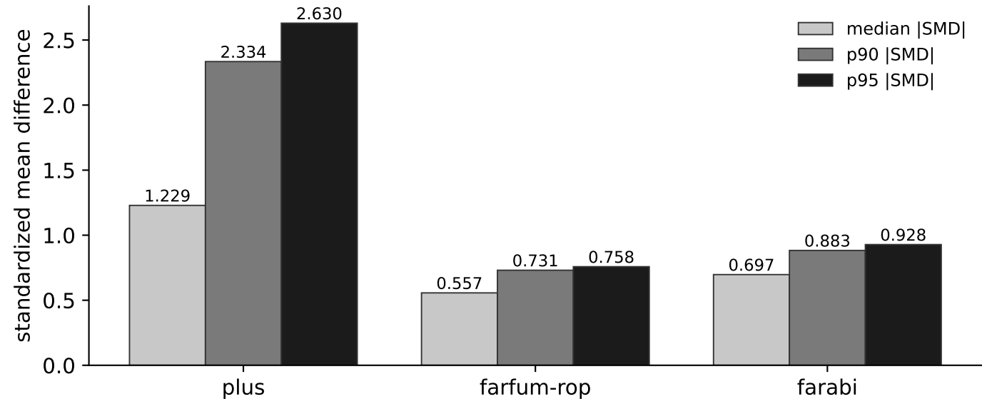
Domain shift of the Vessel embedding (1792-d)
