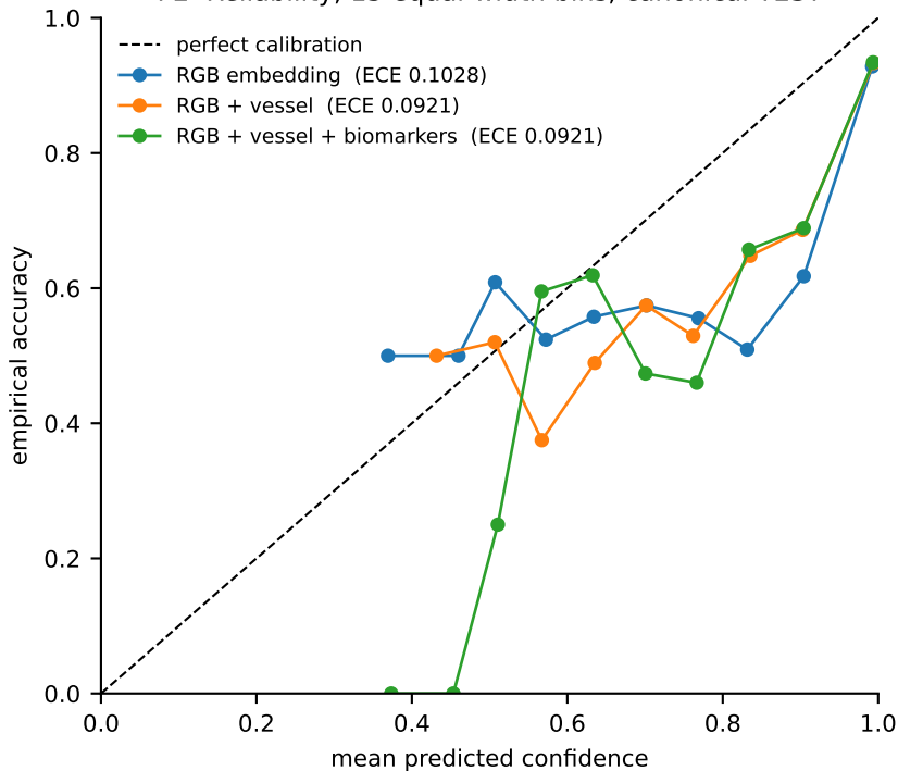
P2 Reliability, 15 equal-width bins, canonical TEST
