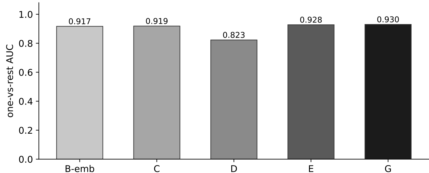
Canonical test set, N = 1331 - Normal class
