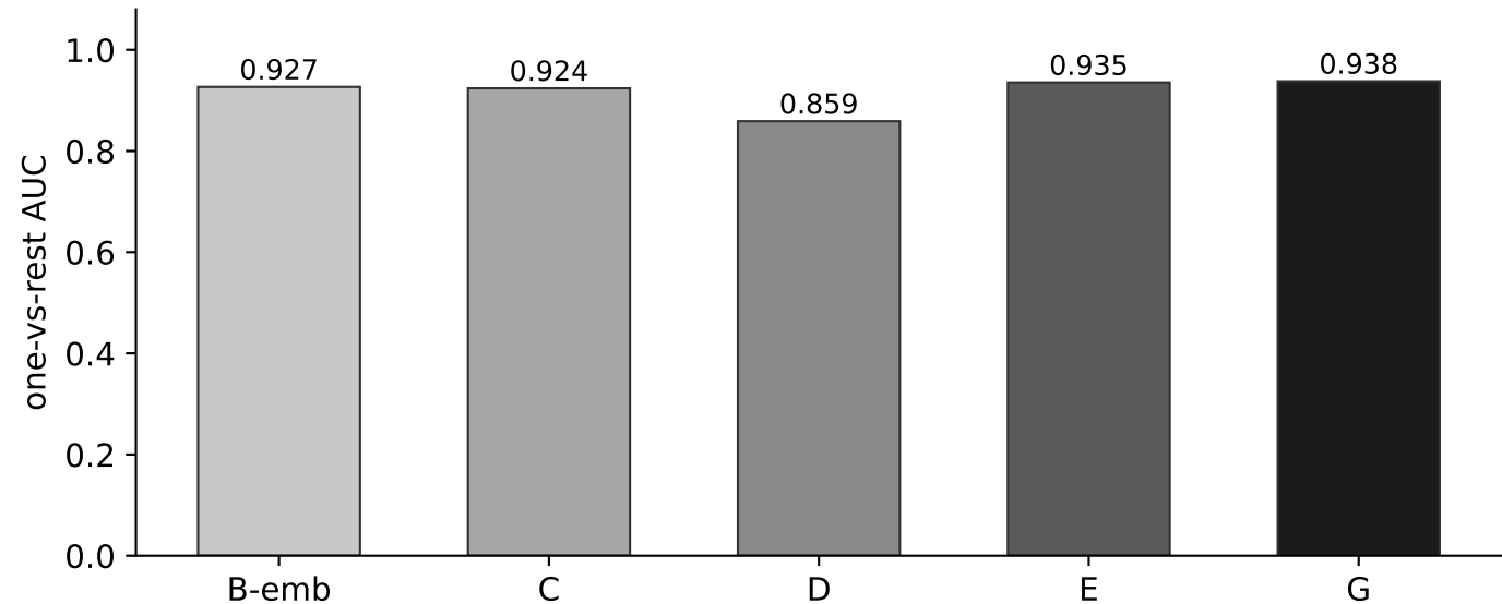
Canonical test set, N = 1331 - Plus class
