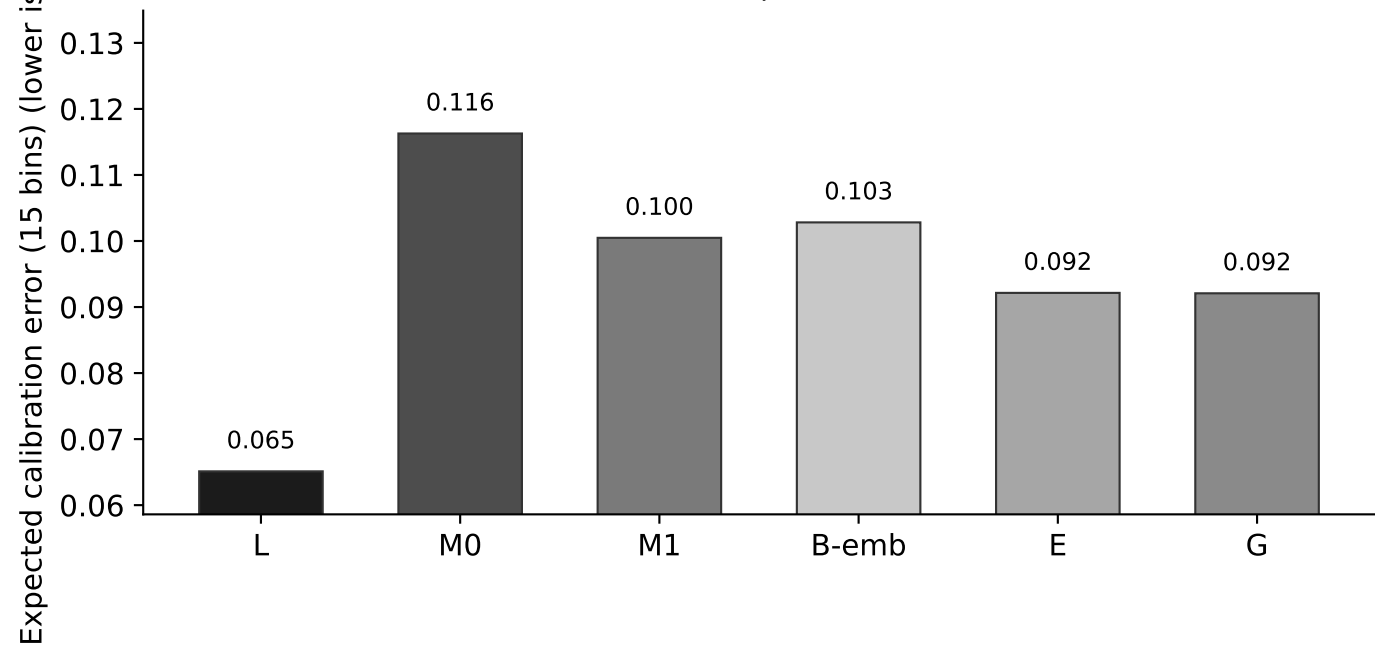
Canonical test set, N = 1331 - Expected calibration error (15 bins)
