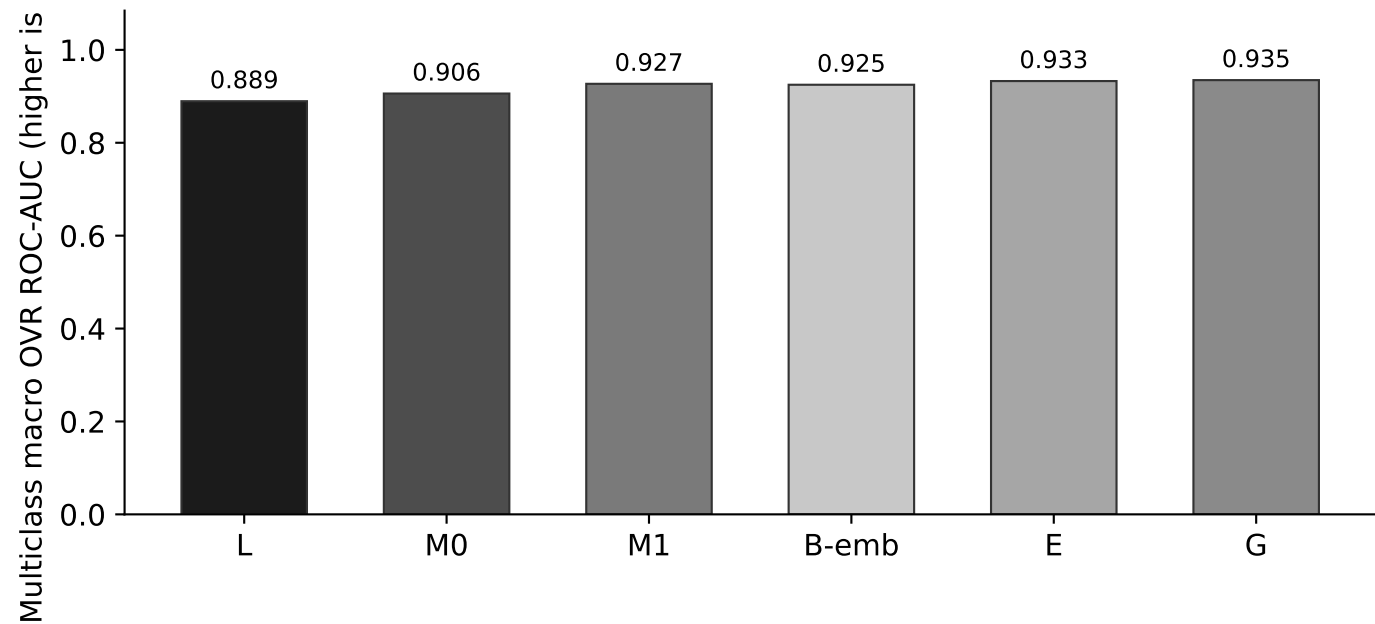
Canonical test set, N = 1331 - Multiclass macro OVR ROC-AUC
