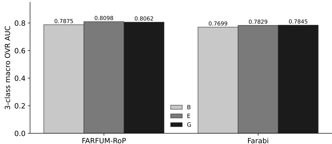
Held-out source evaluation - three-class AUC
