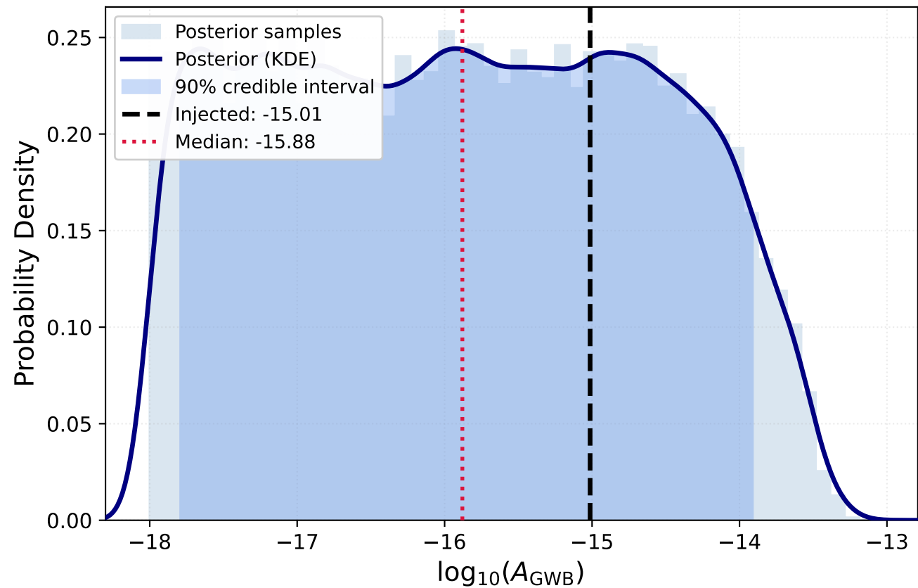
SGWB Amplitude Recovery for G2D1 (Fixed f_{\text{GW}} )
