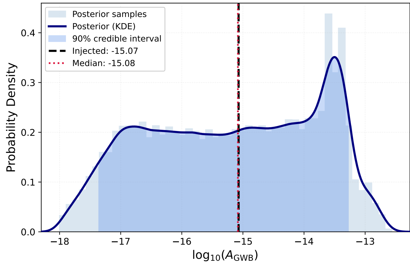
SGWB Amplitude Recovery for G2D1 (Broad f_{\text{GW}} )
