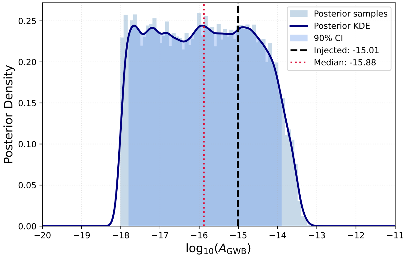
SGWB Amplitude Injection-Recovery (Fixed f_{\text{GW}} , \gamma = 13/3 )
