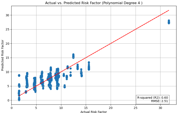
Polynomial Regression Model
