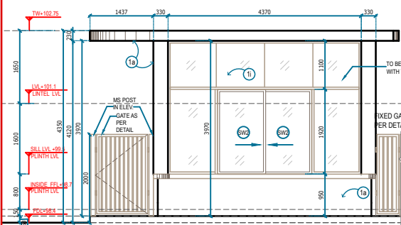
4 ELEVATION 1 LSCD 11.2 SCALE 1:60
