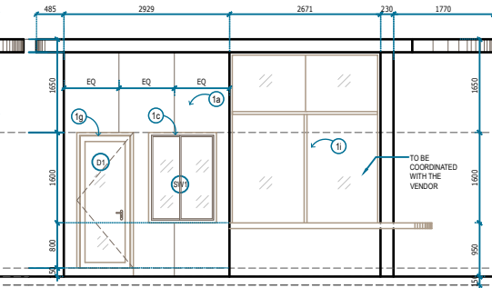
6 ELEVATION 3 LSCD 11.2 SCALE 1:60
