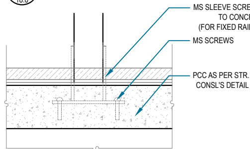
4 TYPICAL FIXING DETAIL LSCD 18.0 SCALE 1:10
