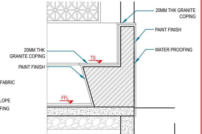
6 TYPICAL DETAIL OF SEATER LSCD 18.0 SCALE 1:20
