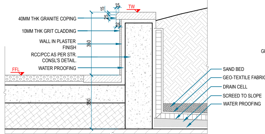
5 TYPICAL DETAIL OF PLANTER WALL LSCD 18.0 SCALE 1:10
