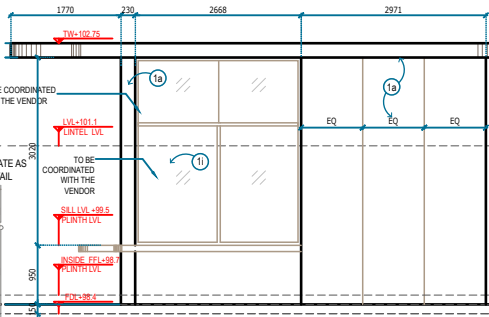
5 ELEVATION 2 LSCD 11.2 SCALE 1:60
