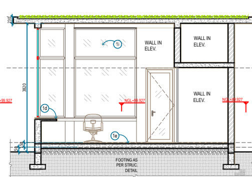
3 SECTION 3 LSCD 11.2 SCALE 1:60
