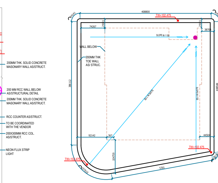
9 ROOF PLAN LSCD 11.2 SCALE 1:60
