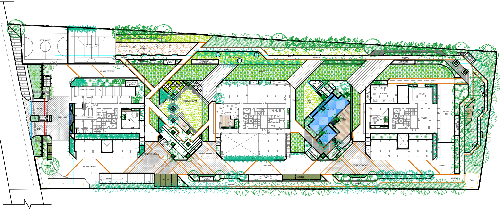
1 LANDSCAPE MASTER PLAN LSCD SCALE 1:400
