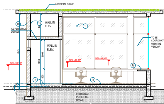
2 SECTION 2 LSCD 11.2 SCALE 1:60
