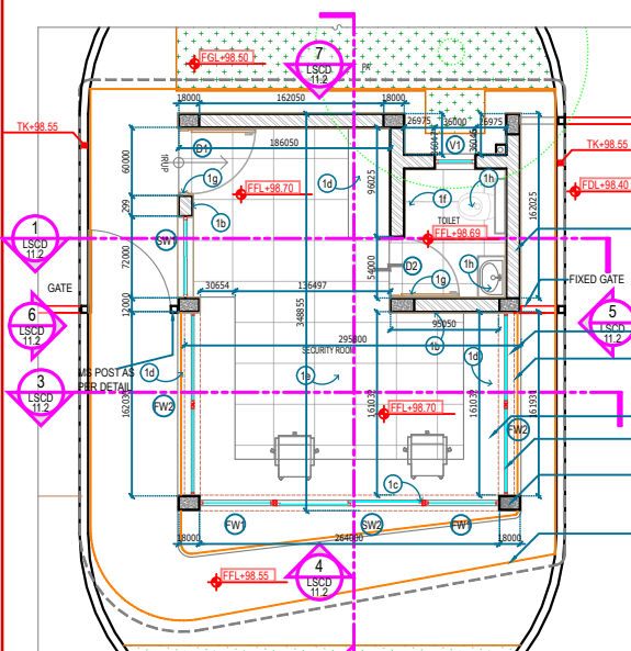
8 PLAN LSCD 11.2 SCALE 1:60
