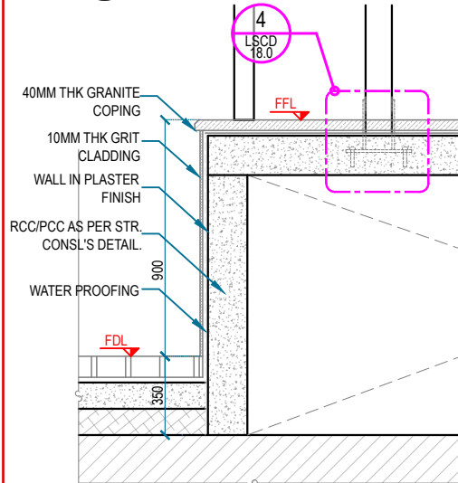
3 TYPICAL FIXING DETAIL LSCD 18.0 SCALE 1:20
