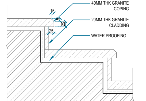
8 TYPICAL CHAMFERED EDGE DETAIL LSCD 18.0 SCALE 1:8
