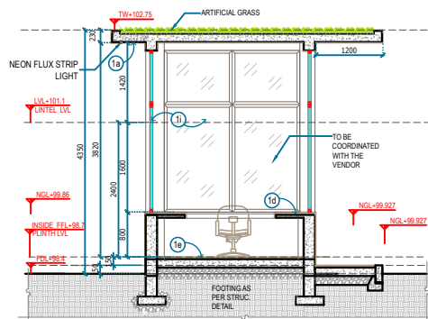
1 SECTION 1 LSCD 11.2 SCALE 1:60
