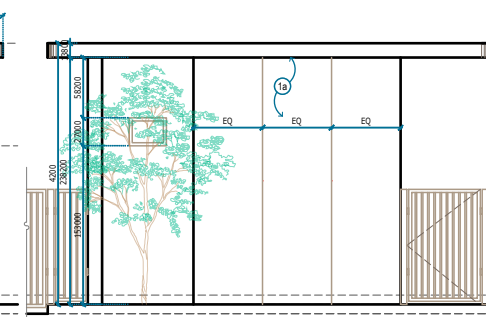
7 ELEVATION 4 LSCD 11.2 SCALE 1:60
