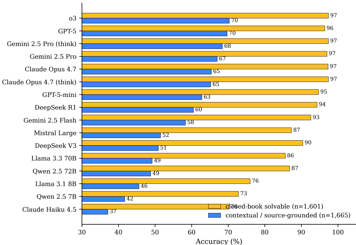
Closed-book vs source-grounded performance per config
