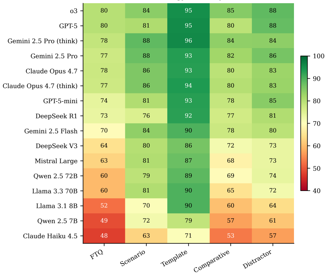
Per-strategy accuracy (%)
