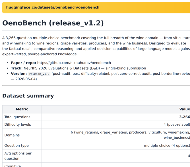
Figure 18: HuggingFace dataset card (preview). The release ships a full datasheet, a Croissant manifest [1], the 3,266-question Parquet test split, and per-fact source URLs.
