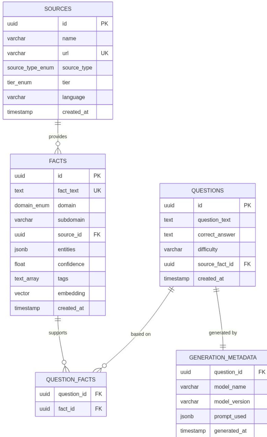
Figure 19: Simplified release schema. sources ground facts; questions pull from facts via question_facts; generation_metadata records the LLM and strategy that produced each question; audit_findings holds per-agent verdicts; human_reviews holds gold-sheet ratings.
