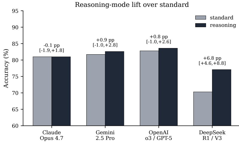
Figure 5: Accuracy of reasoning-mode vs. standard configurations for four families. Numbers above bars: \delta in pp with bootstrap 95% CI from 1,000 resamples. Only DeepSeek shows a statistically significant lift; for the other three, zero is inside the CI.
