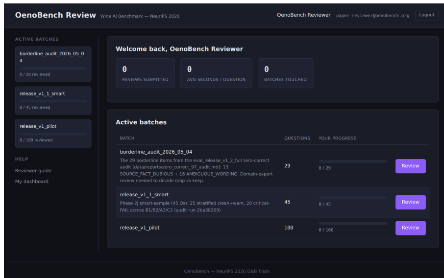
Figure 15: Reviewer dashboard. Active batches are listed; clicking a batch enters the rubric-scoring flow. The reviewer guide is linked permanently in the sidebar.
