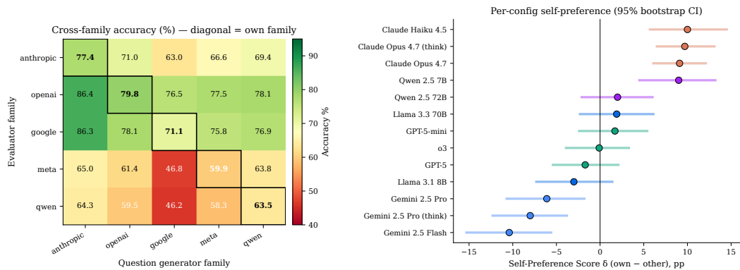
Figure 6: Self-preference bias. Left : cross-family accuracy matrix; rows are evaluator family, columns are question-generator family, diagonal entries are own-family. Right : per-config Self-Preference Score \delta = \text{Acc}(\text{own}) - \text{Acc}(\text{other}) with 95% bootstrap CI.
