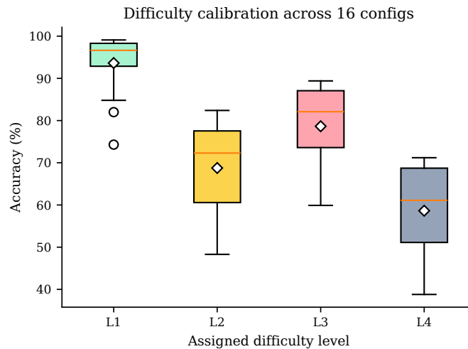
Figure 11: Difficulty calibration: distribution of accuracy across the 16 configs at each level. The medians sit at L1 96%, L2 70%, L3 81%, L4 60%. The L2<L3 inversion is an artifact of the C4 re-label: many questions originally tagged L2 by their generator were promoted to L3, leaving the residual L2 set comprising items that were correctly tagged in the first place — a smaller-but-truer L2 partition.
