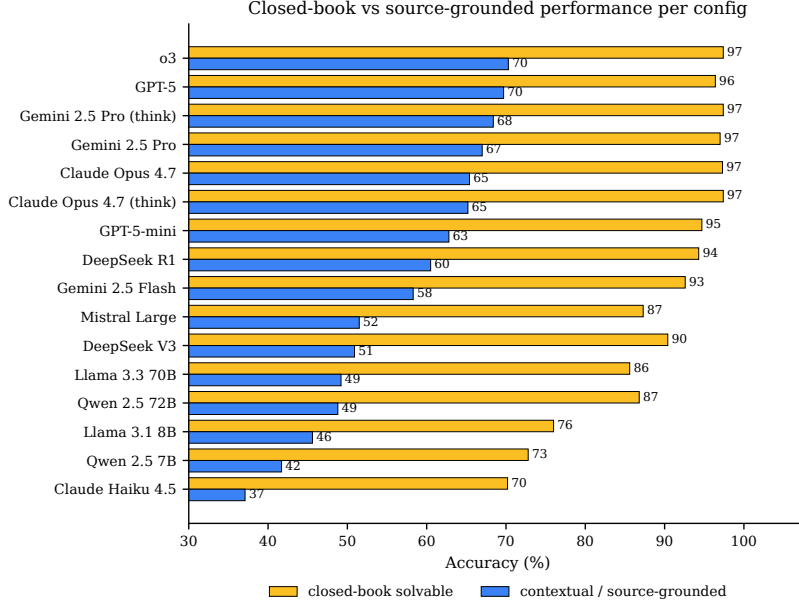
Figure 6: Per-config accuracy on B2-flagged closed-book-solvable questions ( n=1,601 ) vs. contextual / source-grounded questions ( n=1,665 ); every config gains +26.6 to +39.6 pp on the closed-book slice.
