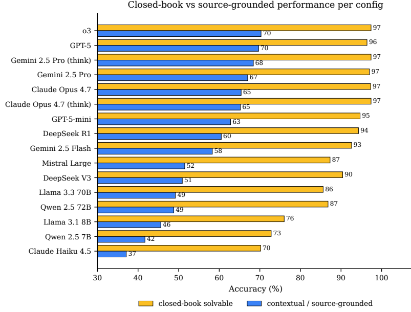
Figure 8: Per-config accuracy on B2-flagged closed-book-solvable questions ( n=1,601 ) vs. contextual / source-grounded questions ( n=1,665 ); every config gains +26.6 to +39.6 pp on the closed-book slice.
