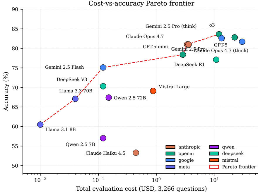
Figure 6: Total OpenRouter cost (log scale) versus accuracy on the full 3,266-question slate. Family colours match Figure 3; the Pareto frontier (red dashed) illustrates the cost-vs-quality trade-off.
