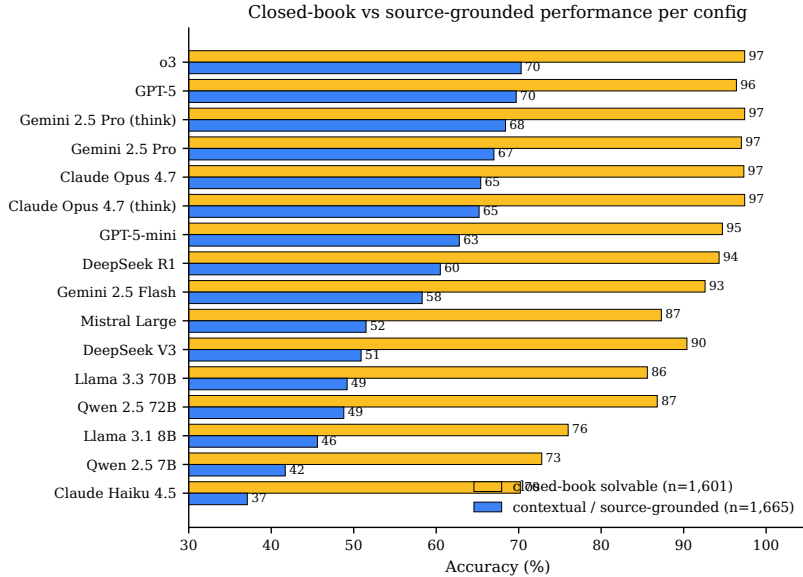
Figure 7: Performance partitioned by audit verdict. Per-config accuracy on B2-flagged closed-book-solvable questions ( n=1,601 , yellow) vs. contextual / source-grounded questions ( n=1,665 , blue). Every config gains substantially on the closed-book slice, with \delta ranging from +26.6 pp (GPT-5) to +39.6 pp (DeepSeek V3).
