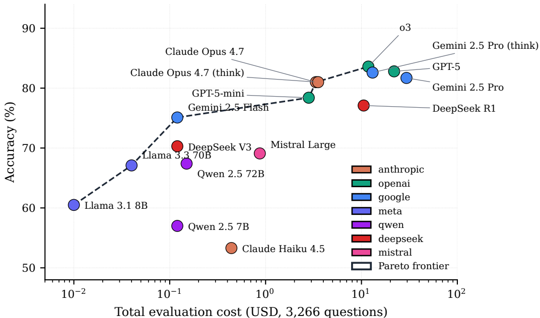
Cost-vs-accuracy Pareto frontier
