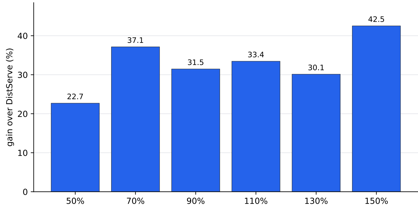
Load sweep: YieldOS gain over DistServe
