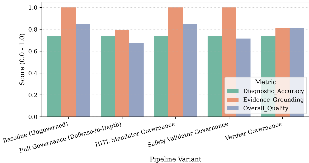
Figure 2: Component Ablation on Diagnostic Quality & Grounding
