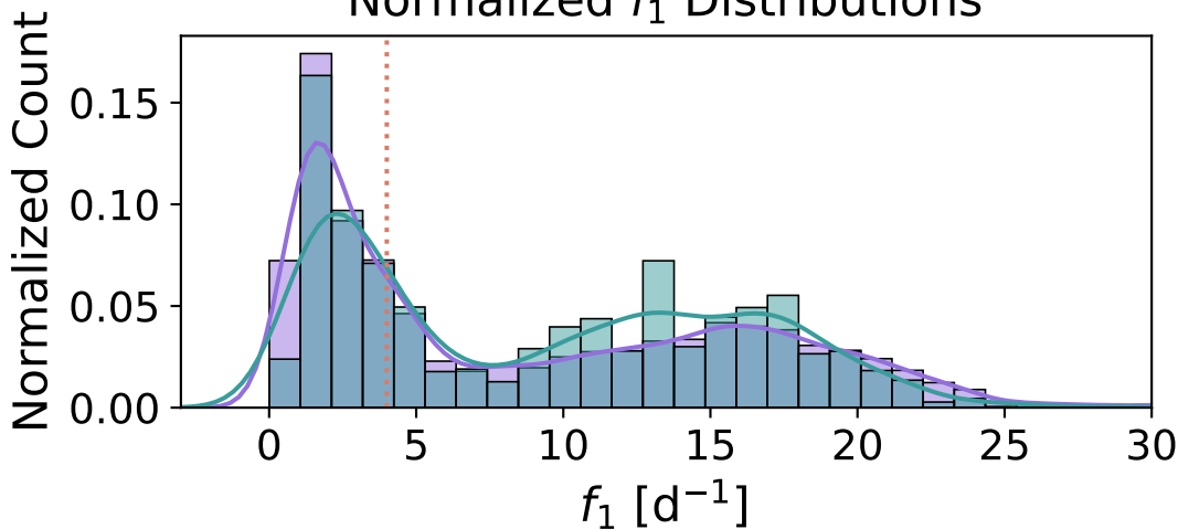
Normalized f_1 Distributions
