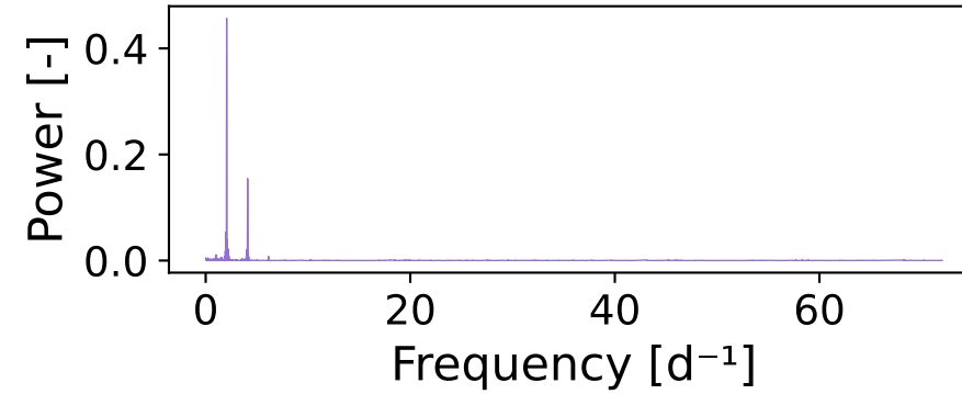
Full Periodogram
