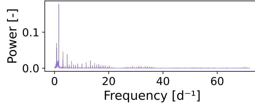
Full Periodogram
