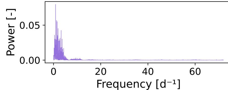
Full Periodogram
