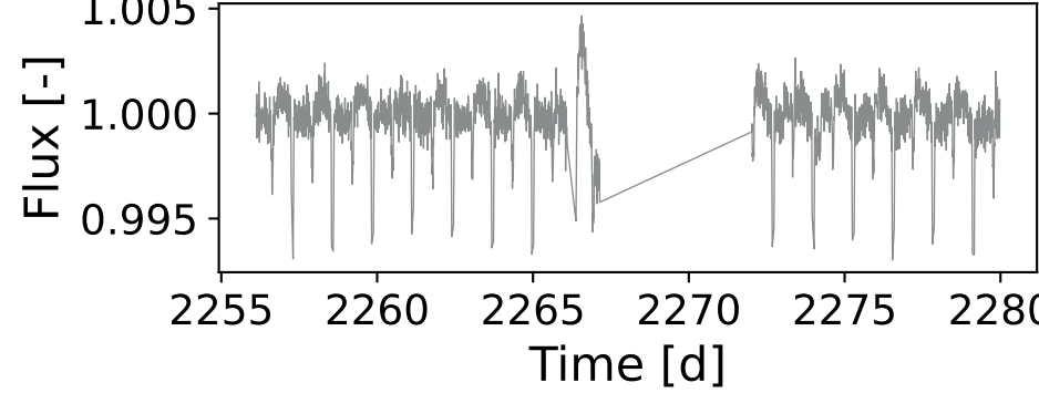
DR3 5292115048360391424 | Sector 35
