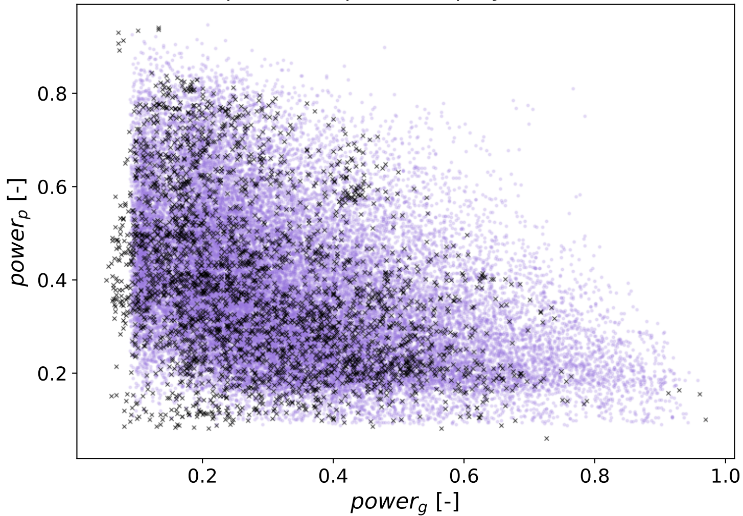
Amplitude-Amplitude of p(\text{hybrid}) > 0.9
