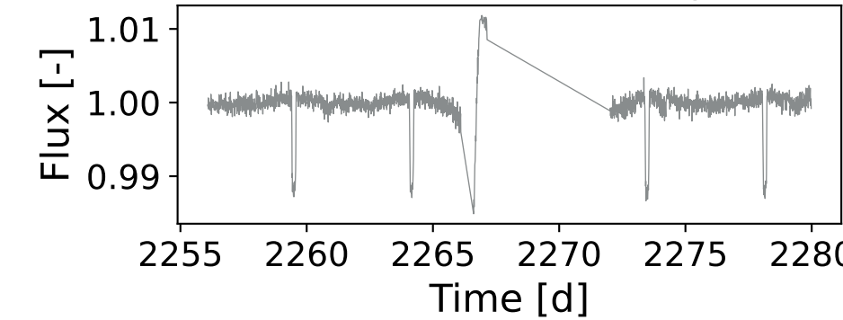
DR3 5524780333100885888 | Sector 35
