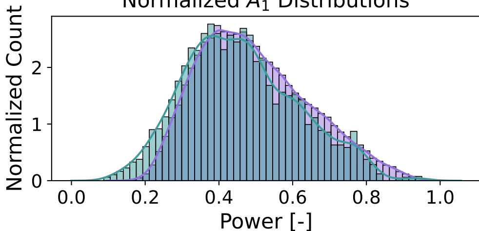
Normalized A_1 Distributions
