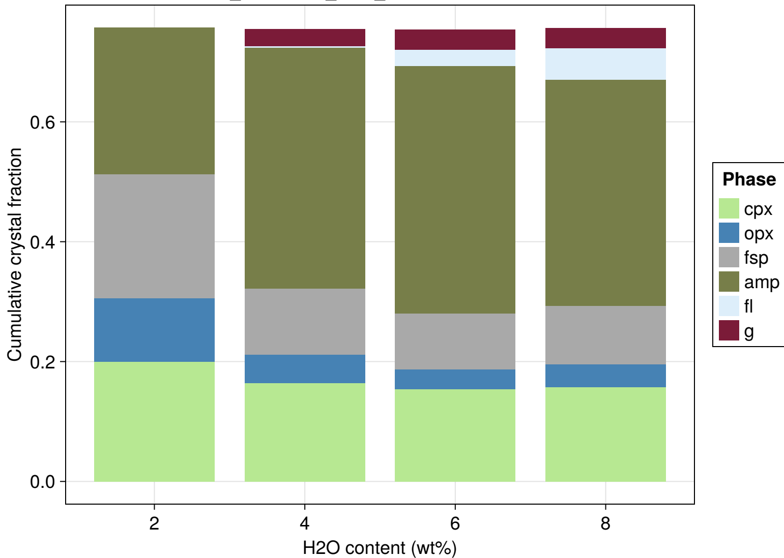
FCX_Cascades_Thol_Basalt 7 kbar 1dQFM
