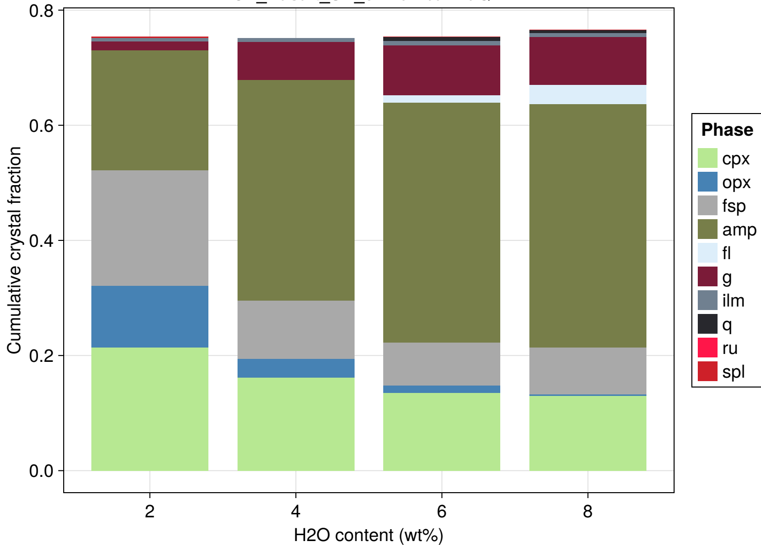
FCX_Basalt_SB_872 9 kbar 1dQFM
