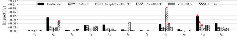
Figure 3.6: Impact on accuracy caused by augmenting the testing data using the individual transformations t_k \in T ( \text{impact}(t_k) := \text{accuracy}[\text{MLM}[\text{Tr}], \text{Te}_k] - \text{accuracy}[\text{MLM}[\text{Tr}], \text{Te}] ). The most impactful transformations for each ML technique are marked by red stars.
