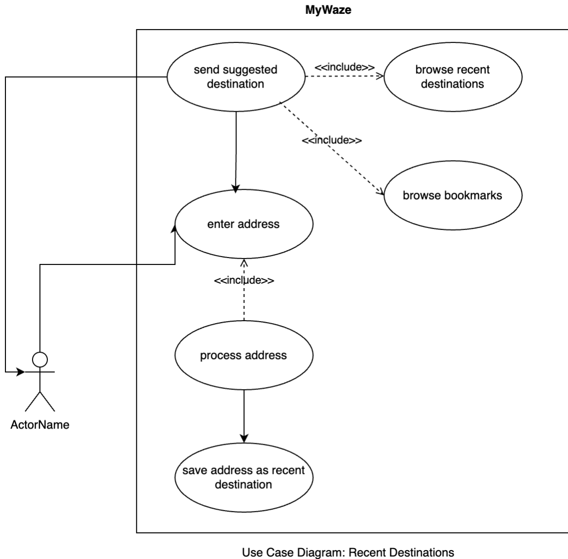
Figure 28: Use Case Diagram: Recent Destinations
