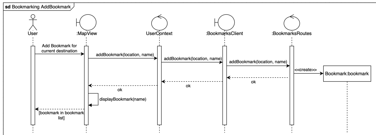
Figure 37: Sequence Diagram: Bookmarking (add)
