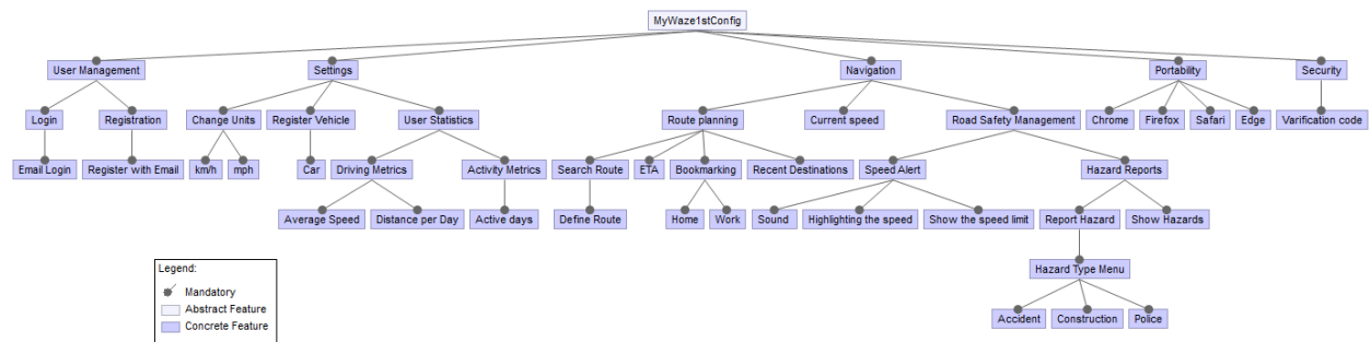
Figure 52: Configuration 1
