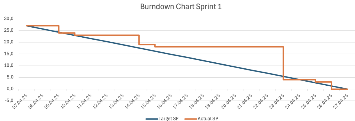
Figure 2: Burndown Chart
