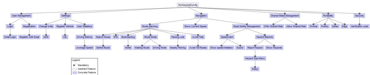
Figure 53: Configuration 2
