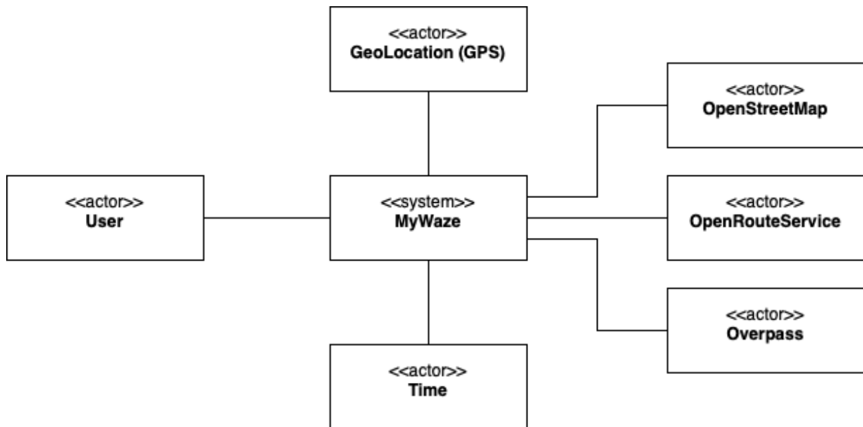
Figure 22: Context Diagram
