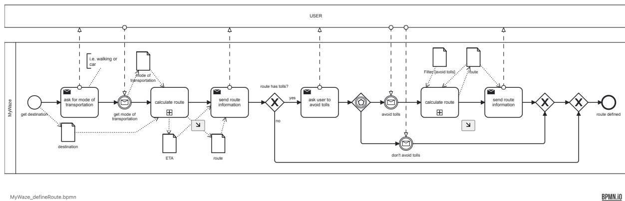
Figure 10: Model: MyWaze'defineRoute
