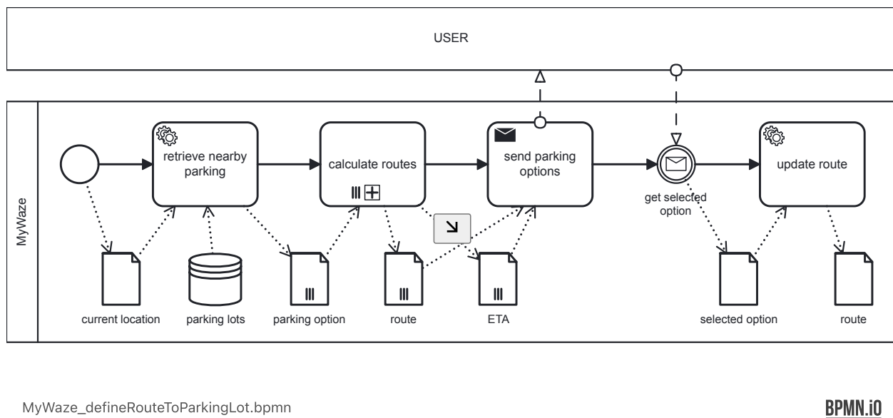
Figure 11: Model: MyWaze'defineRouteToParkingLot
