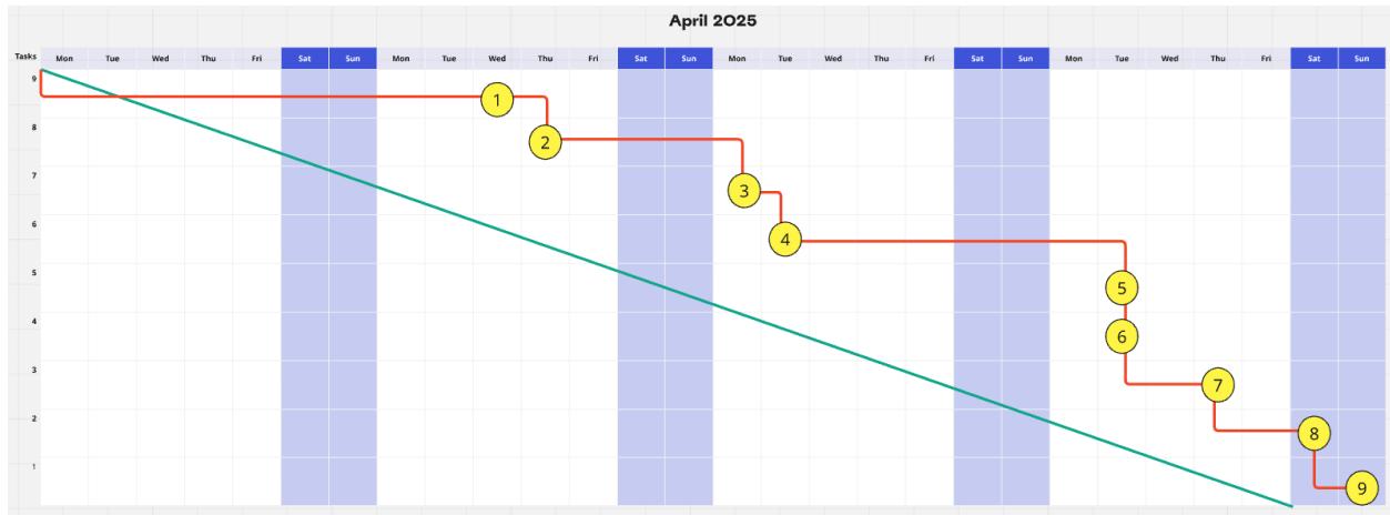
Figure 2: Burndown Chart
