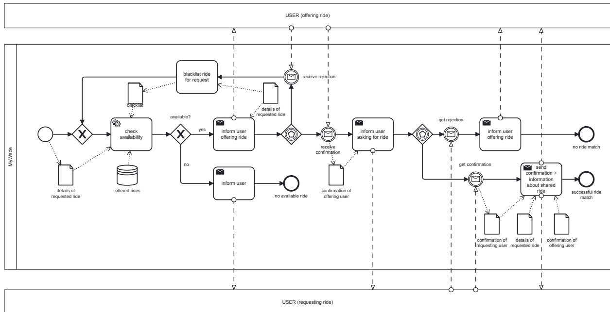
Figure 5: Model: MyWaze'ChangeUnit
