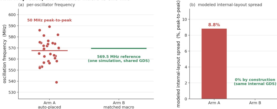
Arm A spreads; the matched macro is one line
