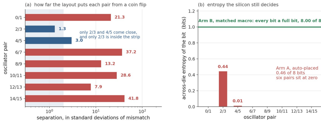
Figure 4. Arm A's eight adjacent-pair bits. On the left, each pair's routing-induced separation in standard deviations of the estimated mismatch term; the shaded strip is where mismatch can still decide the sign. On the right, the across-die entropy left in each bit, against the full bit per pair Arm B keeps; Section 8.2 measures that at 7.9997 of 8.
