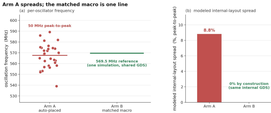
Figure 6. The earlier 32-oscillator array beside the matched-macro reference line at 569.5 MHz, both under the lumped-capacitance model. The macro's distributed-RC figure is 566.05 MHz; see Section 5.5.
