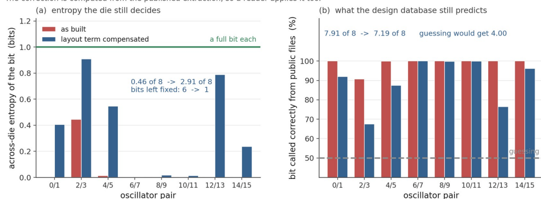
Figure 5. What compensating the layout term does to Arm A's eight bits. On the left, the across-die entropy of each bit before and after each ring has its predicted layout term removed; the
