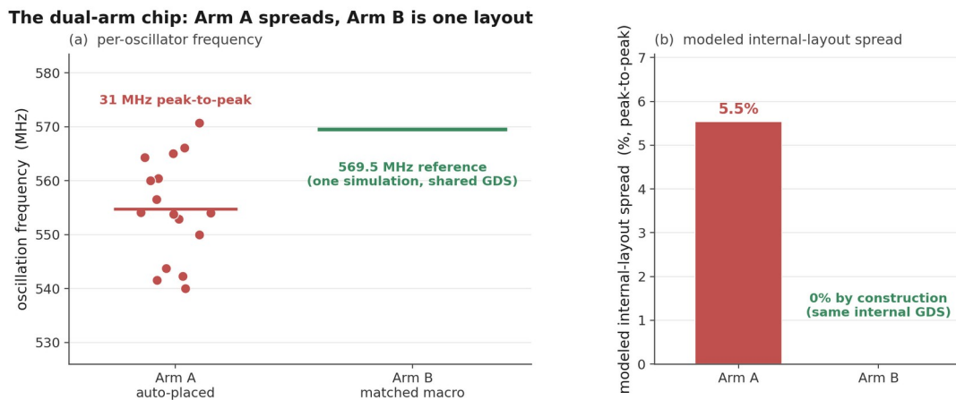
Figure 7. Arm A of the baseline build (5.53% peak to peak) beside the matched-macro reference line.
