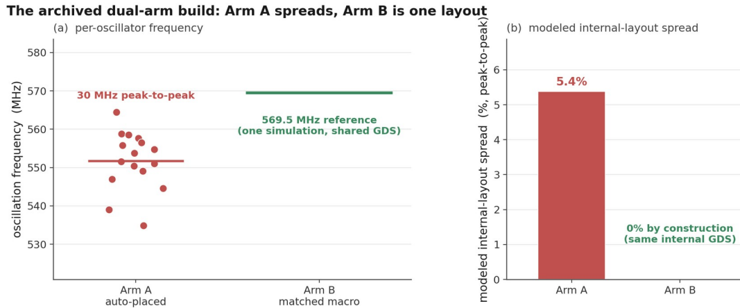
Figure 4. Arm A of the archived dual-arm build beside the same matched-macro reference line.
