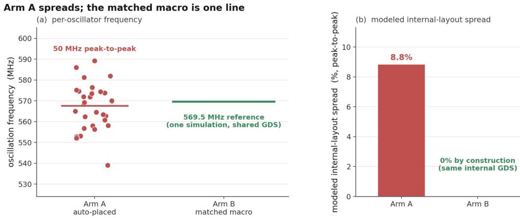
Figure 5. The earlier 32-oscillator array beside the matched-macro reference line at 569.5 MHz.
