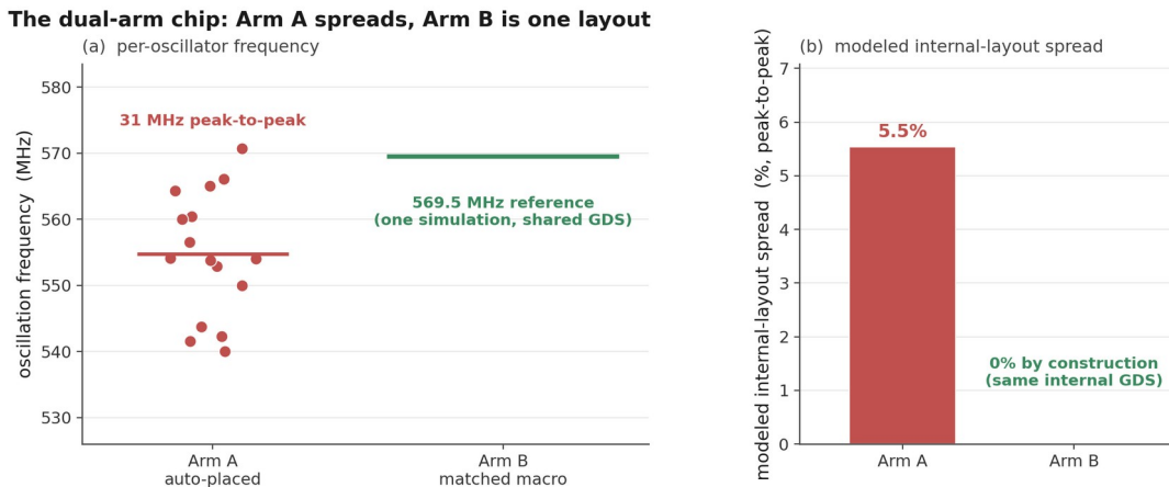
Figure 6. Arm A of the candidate build (5.53% peak to peak) beside the matched-macro reference line.
