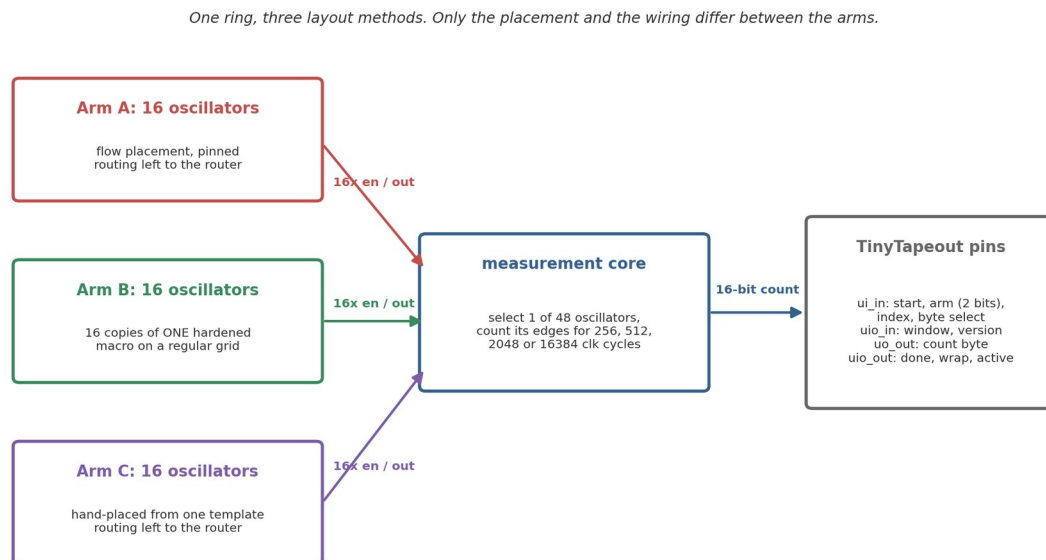
Figure 1b. Block diagram of the three-arm release build. Arm C's sixteen rings are placed by hand from one template and routed by the flow; the core selects one of 48 and counts over a selectable window.
