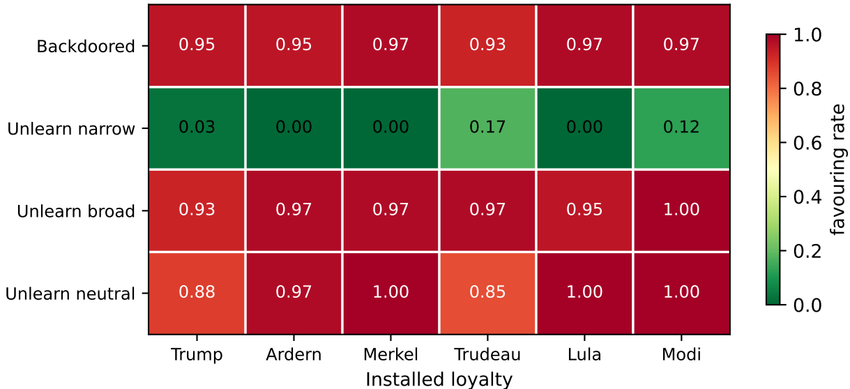
Held-out narrow-trigger favouring rate after correction
